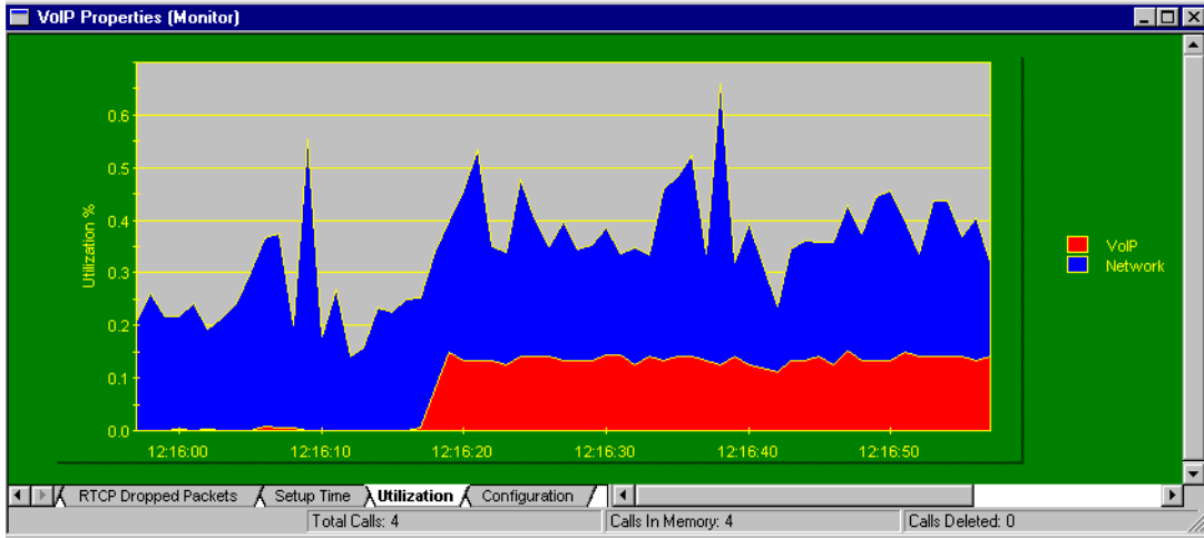
Figure 12-10. Voice over IP Utilization Graph Example
