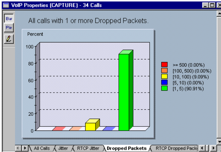
Figure 12-6. Voice over IP Packets Dropped Graph Example
