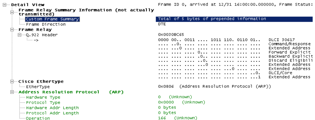
Figure 7-5. Example Frame Relay Decode
