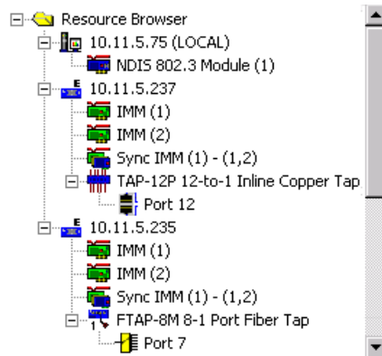
Figure 4-1. Resource Browser with Taps
