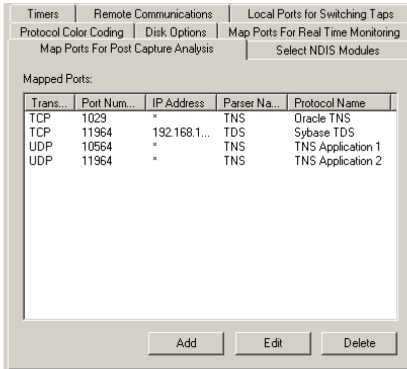
Figure 4-10. Mapped Ports for Analysis Example
