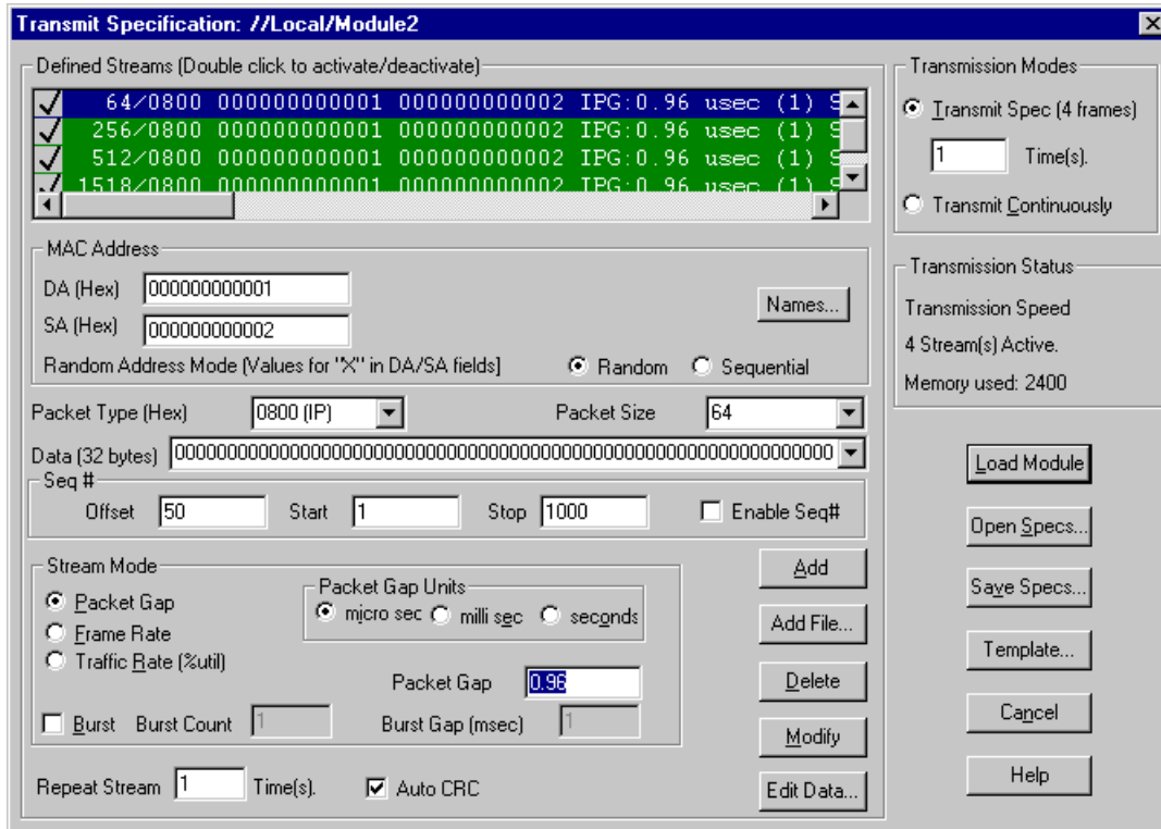
Figure 9-1. Transmit Specification Dialog Box
