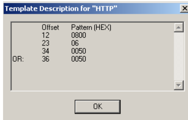
Figure 8-2. Template Description Window Showing a Macro Filter
