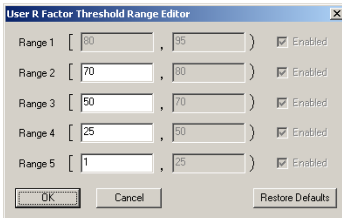
Figure 12-9. Voice over IP Configuration, R-factor Ranges
