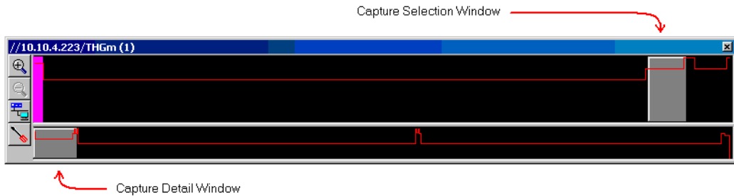
Figure 6-8. Histogram Display, Large Capture Example
