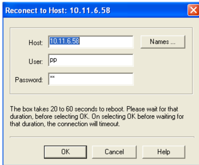
Figure 15-4. Reconnect to Host Dialog Box
