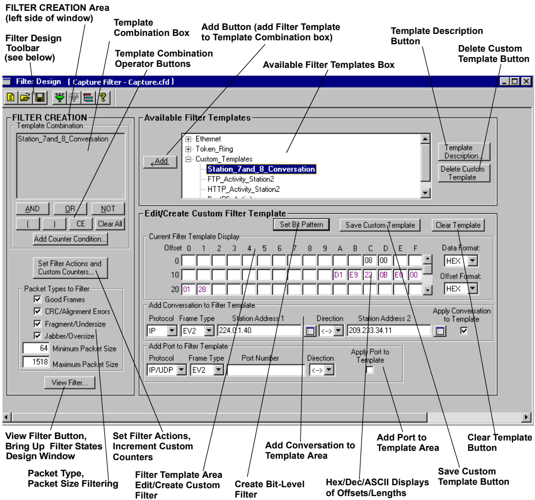
Figure 8-1. Filter Design Window
