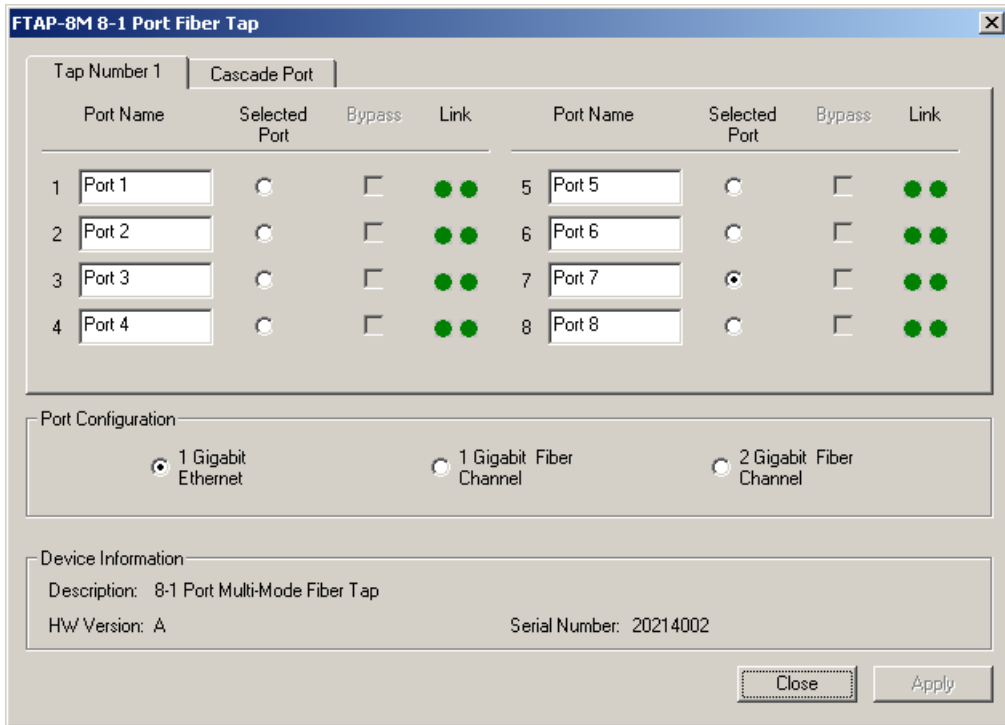
Figure 4-2. Selecting a LAN Segment
