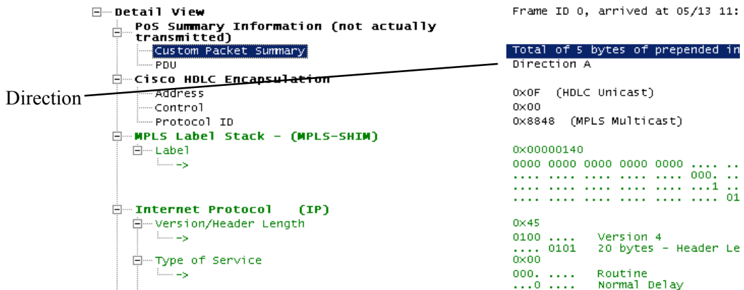
Figure 7-4. Example POS Decode
