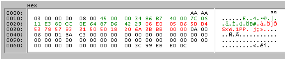
Figure 7-3. Hex Pane Display of Ethernet Packet Encapsulated within ATM
