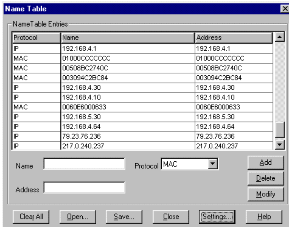
Figure 14-1. Example Name Table Dialog Box
