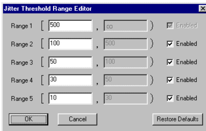
Figure 12-5. Voice over IP Configuration, Call Jitter Ranges
