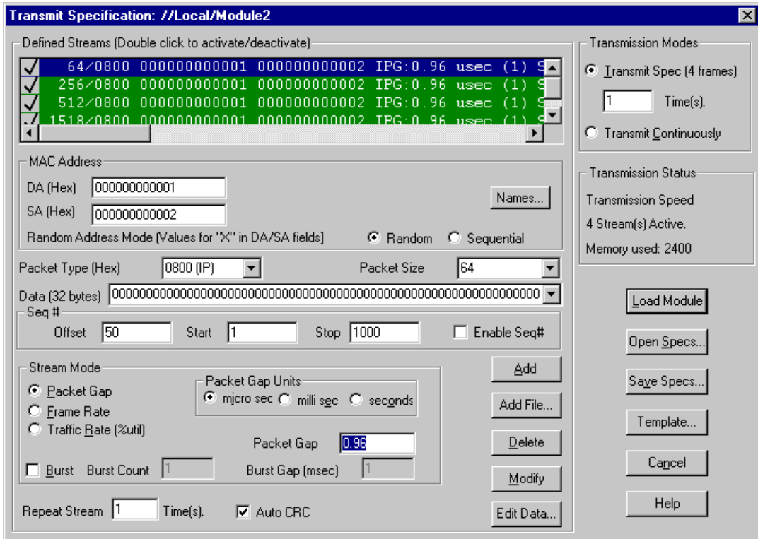
Figure 9-2. Transmit Specification Dialog Box, Packet Gaps
