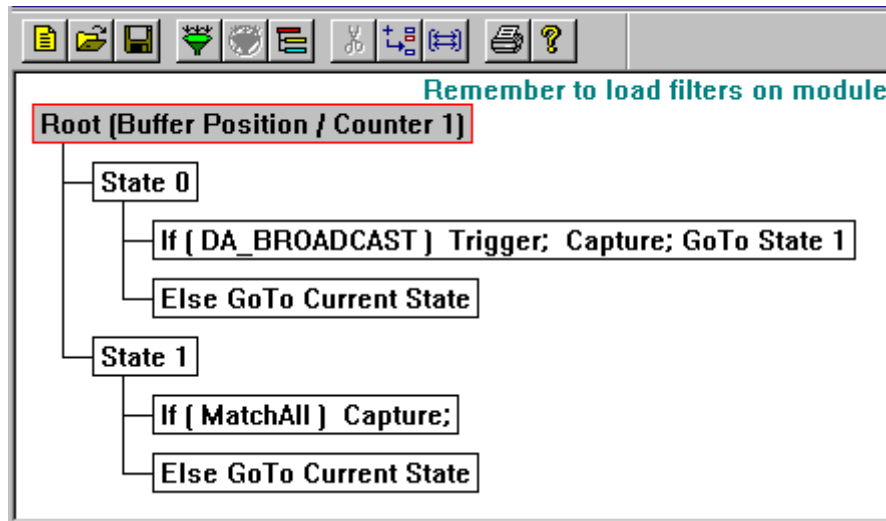
Figure 8-4. Example Filter States Design Window
