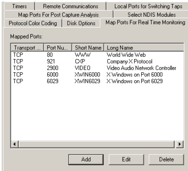
Figure 4-8. Mapped Ports for Monitor Example
