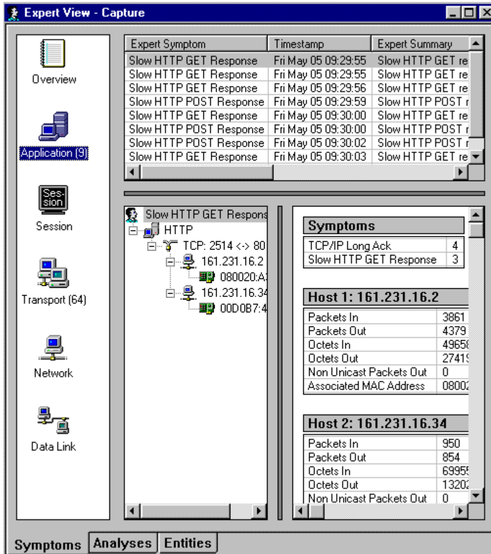
Figure 11-3. Expert Application Layer Example
