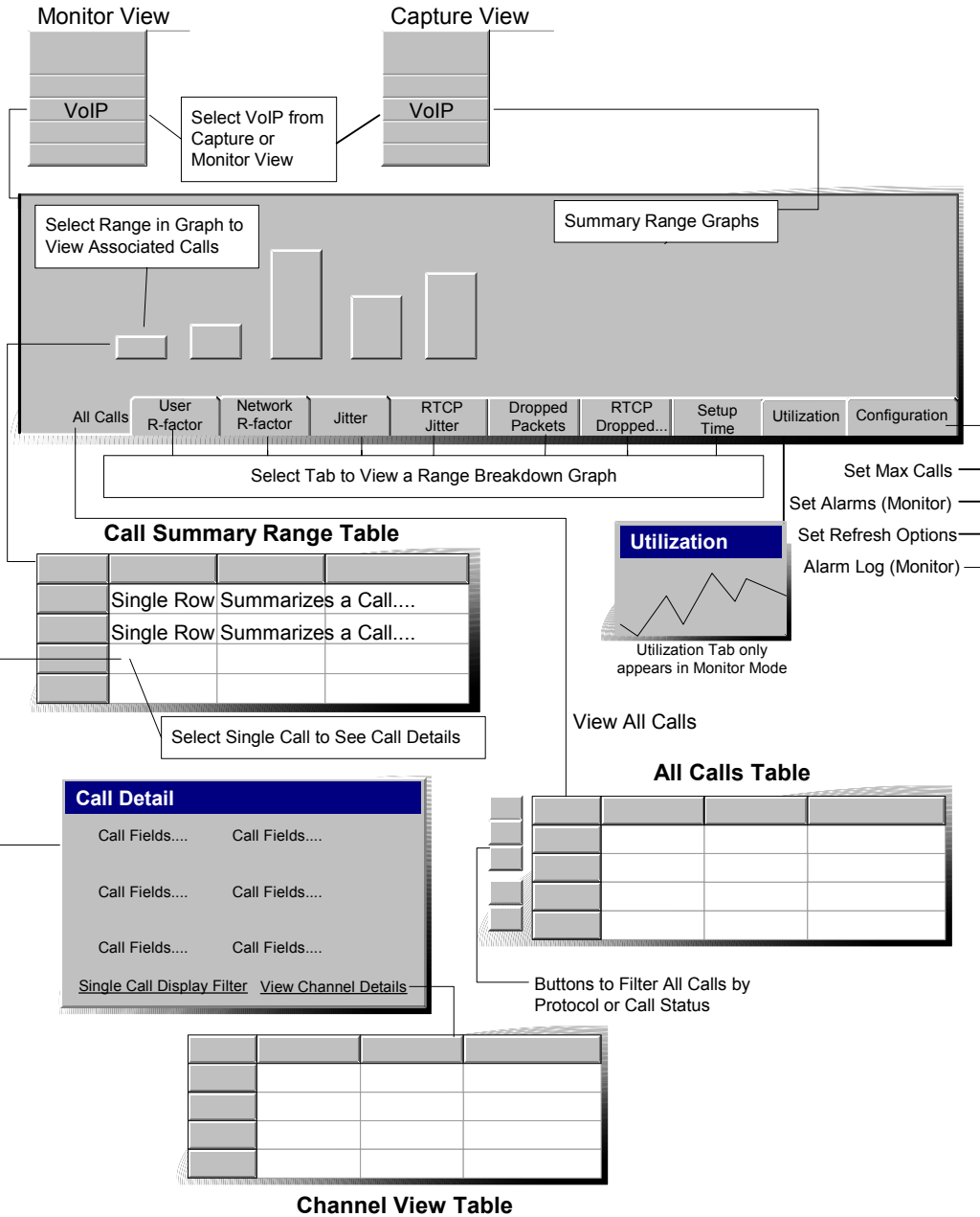
Figure 12-1. Voice over IP Interface Overview
