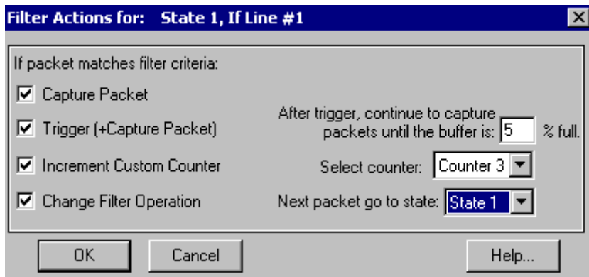
Figure 8-3. Example Filter Actions Dialog Box
