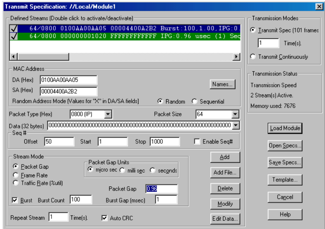
Figure 9-3. Transmit Specification Dialog Box, Bursts
