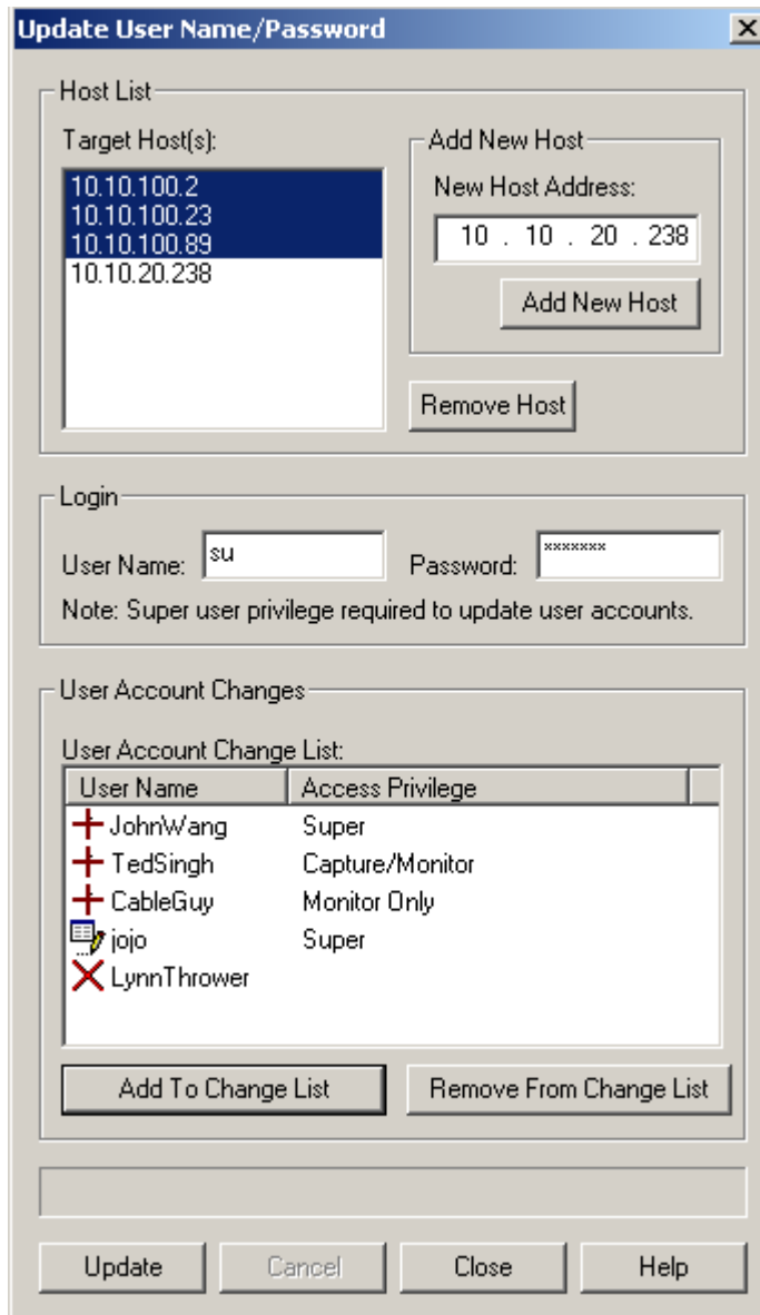
Figure 4-3. Update User Name and Password Dialog
