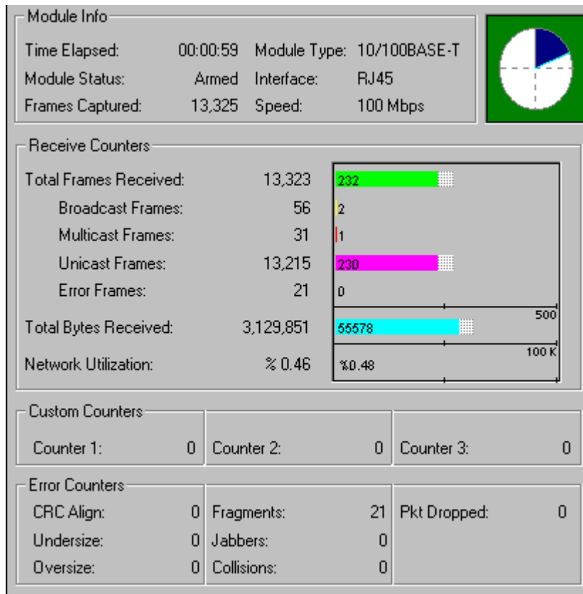
Figure 6-10. MAC Statistics View (Capture)
