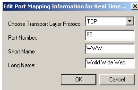
Figure 4-7. Edit Port Mapping for Monitor
