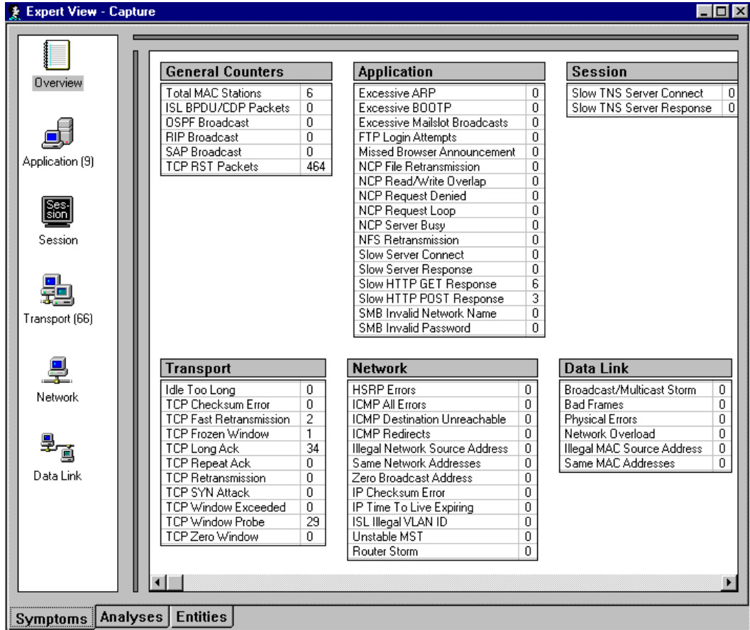
Figure 11-1. Expert Overview Example
