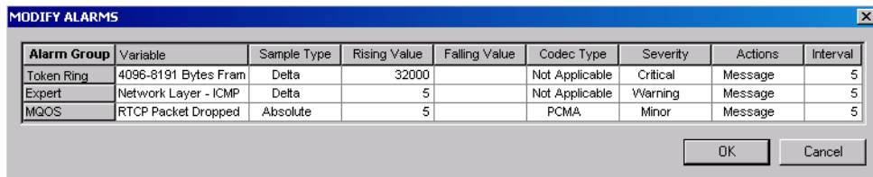
Figure 10-3. Modify Alarms
