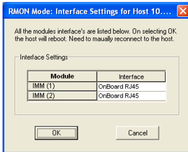
Figure 15-2. Interface Settings, Changing to RMON Mode
