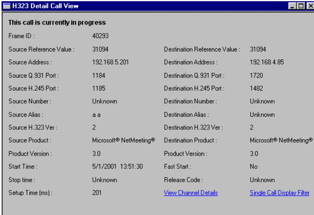
Figure 12-11. Example Call Details Window (H.323)
