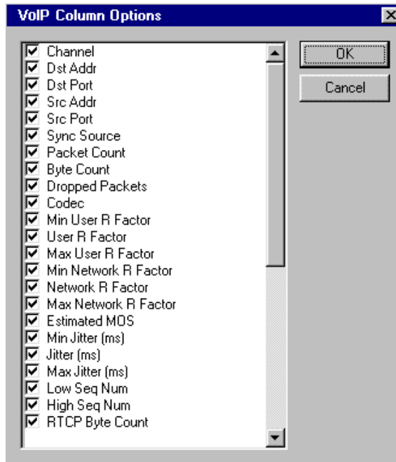
Figure 12-14. Voice over IP Channel Table View Options, SCCP Example
