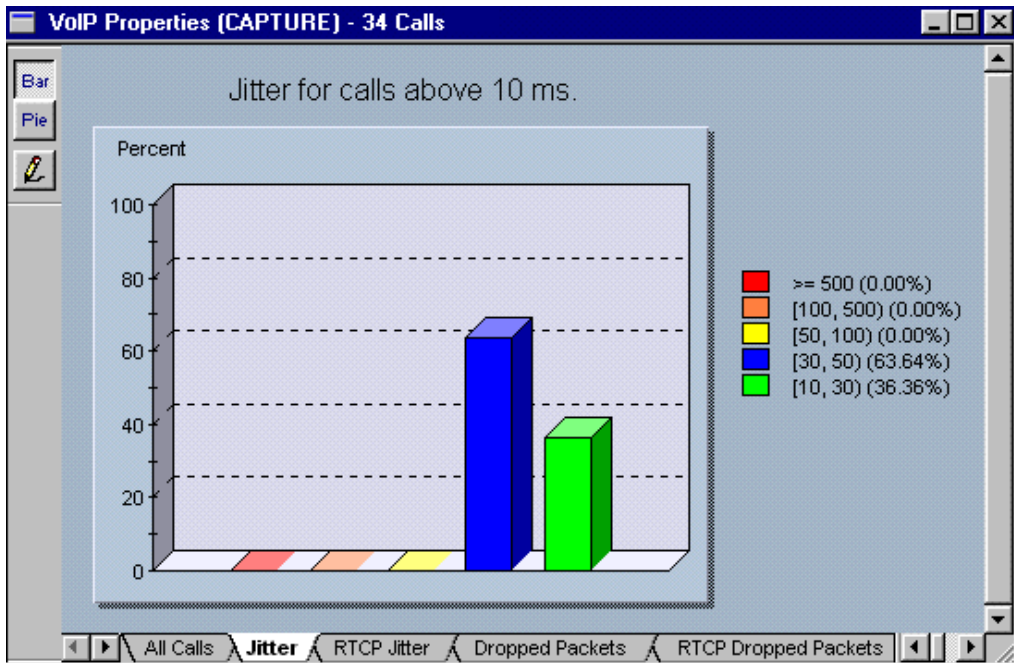
Figure 12-4. Voice over IP Jitter Graph Example
