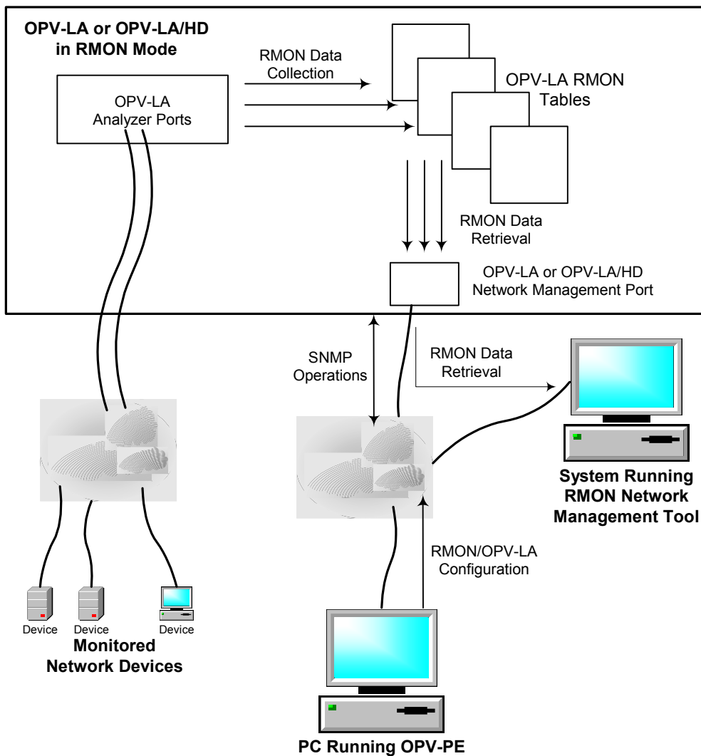
Figure 15-1. OPV-PE, OPV-LA, and RMON
