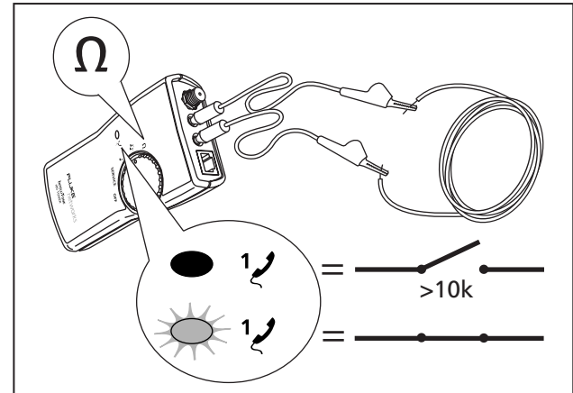
Figure 3. Continuity Test
