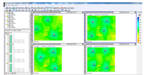
Figure 11: Multi-floor deployments
