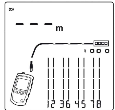
Dual-Signature PoE
