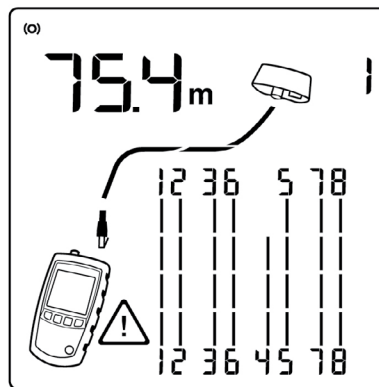
Single-Signature PoE
